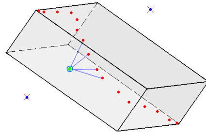
Fig.4. Bounding box of the hit point trajectory modeled with red spots (such as the trajectory of the wrist). The constraint c_r is modeled by the green spot. If the constraint is out of the bounding box of the trajectory (blue dots), the motion which has this trajectory will be discarded, otherwise the distance between the trajectory and the constraint will be calculated.
