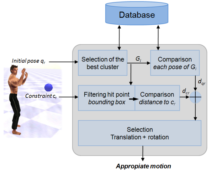
Fig. 5. Overview of the Search algorithm.
