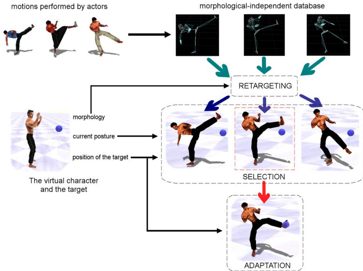
Fig. 2. Synopsis of the morphology independent retrieval and control using an average-size database of motions.
