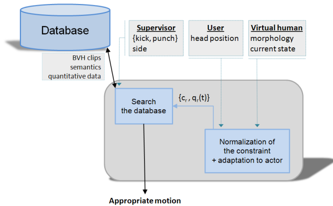
Fig. 3. Overview of the motion retrieval process.
