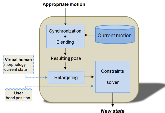
Fig. 6. Overview of the motion adaptation process.
