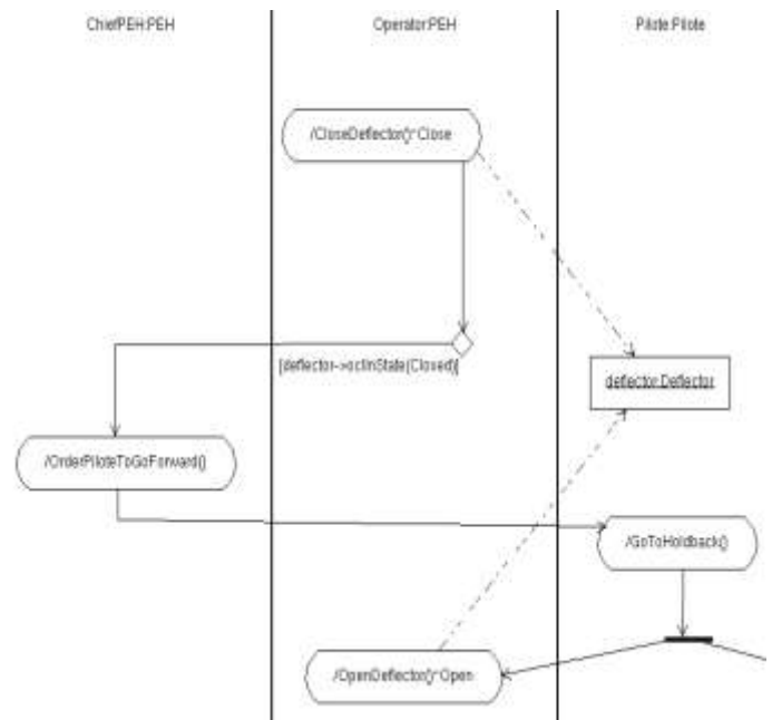
Fig. 8. Example of a procedure written using an activity diagram.
