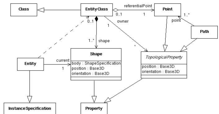
Fig. 4. Class diagram from the Veba metamodel: EntityClass.
