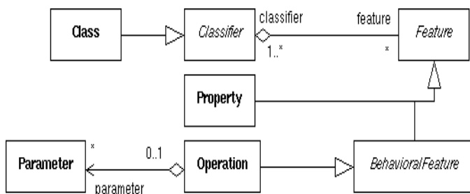
Fig. 3. Class diagram from the Veba metamodel: Features of a Classifier.
