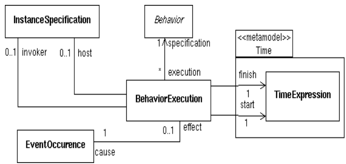
Fig. 5. Class diagram from the Veha metamodel:Behavior::Common package,the BehaviorExecution class.
