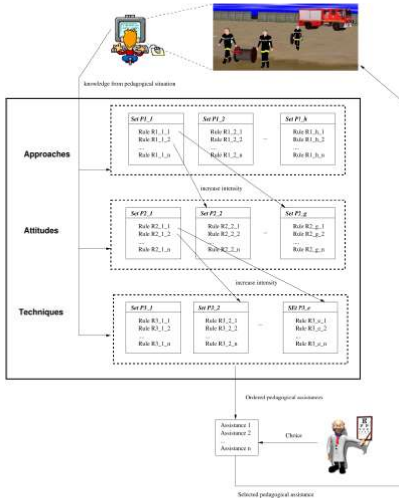
Fig. 9. Complete Representation of the Pedagogical Model.
